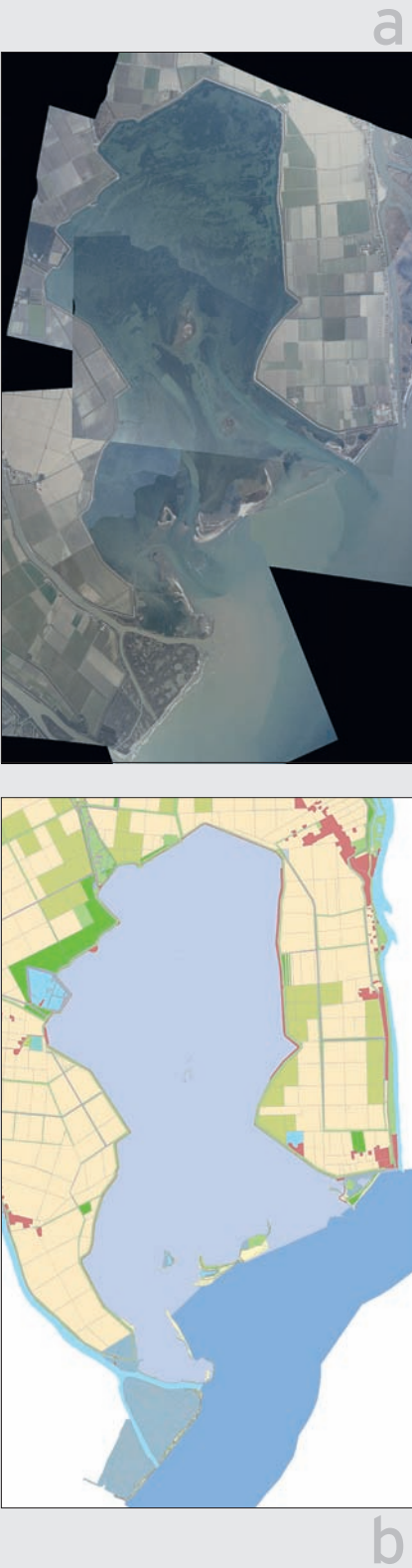
Figure 31: (a) 2008 Delta Po Adige Flight orthophoto (b) on the survey interpretation according to macro-classes of land use (period 1949-2008).
