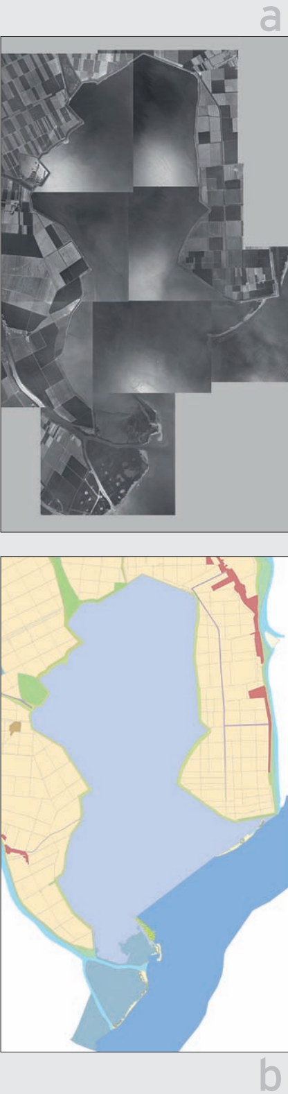
Figure 30: (a) 1983 Veneto Reg. orthophoto and (b) on the survey interpretation according to macro-classes of land use (period 1949-2008).
